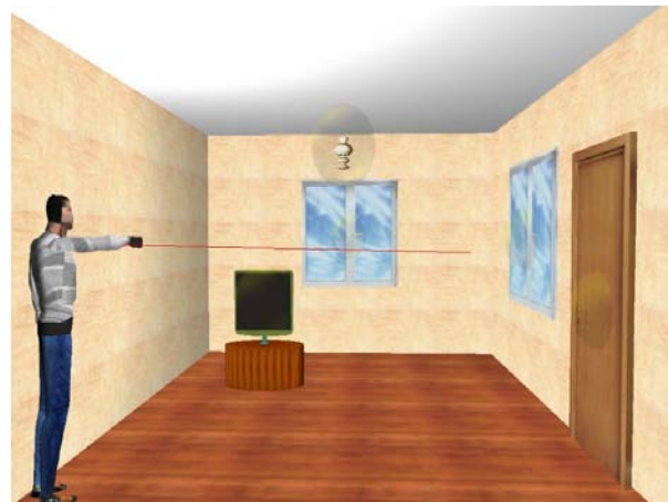
Fig. 2: GUI screenshot
